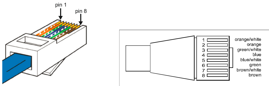
RJ45 pinout details
